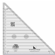
CGRT45
